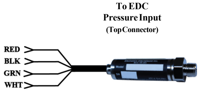
The PT-30GA Pressure Transducer is used on most engines for pressures up to 35 psi.
