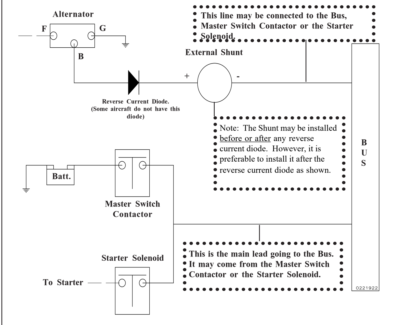
Figure 2: External Shunt Installed in the Alternator Lead
