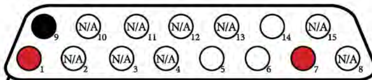
15-Pin D-Sub Connector Wire Side View
