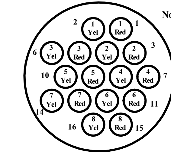
UBG Extension Cable Harness (Left or Right) Back View (wire side)
